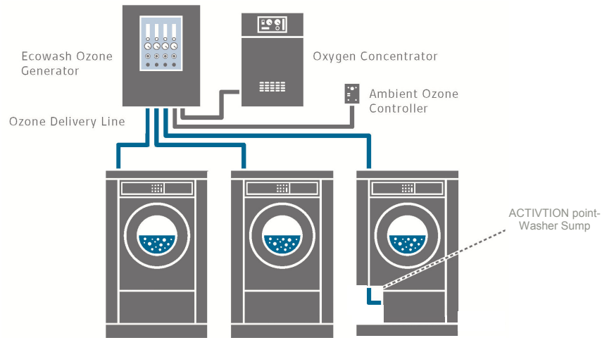
Eco-Wash TRIPLE Washer System EW 200-3
